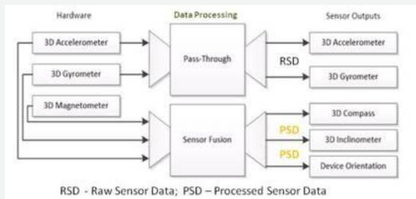
9-Axis Sensor Fusion System (Microsoft – Supporting Sensors in Windows 8)
